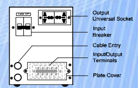
REAR VIEW SES-1H ~ SES-10H
